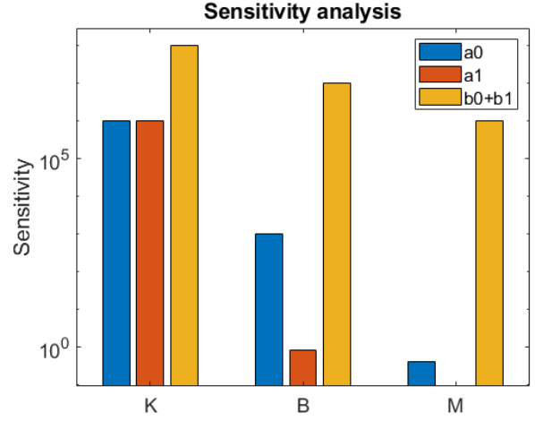
Fig. 6: Local sensitivity analysis \left. \frac{\partial X_i}{\partial Y_j} \right|_{y_0} , on a logarithmic scale, with X_i the impedance parameters and Y_j the discrete coefficients.
